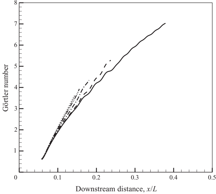
FIGURE 11. Simulations T0–T4: Görtler number on the pressure surface, upstream of transition or separation, G \equiv (\bar{u}_t^\infty \theta / \nu) (\theta / \mathscr{R})^{1/2} . Lines: — T0; - - - T1; — · — T2; ····· T3; ····· T4.
