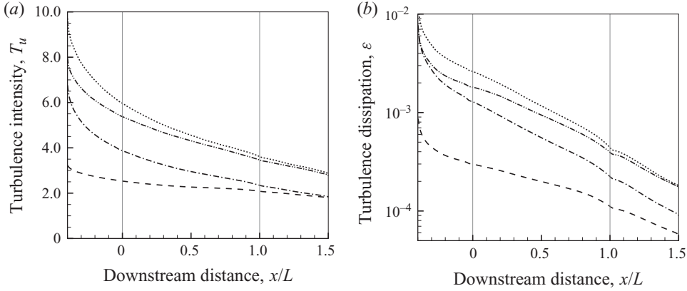
FIGURE 8. Simulations T1–T4. (a) The turbulence intensity and (b) dissipation, plotted at mid-pitch from the various simulations with inflow turbulent forcing. Lines: --- T1; — · — T2; — — — T3; ··· T4.
