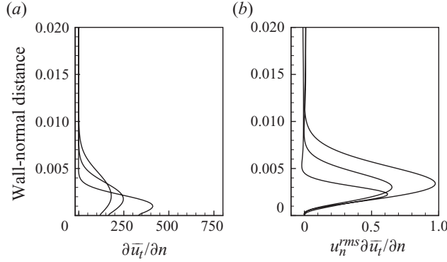
FIGURE 30. Simulation T2, pressure surface. (a) Profiles of \partial \bar{u}_t / \partial n and (b) the product u_n^{rms} \partial \bar{u}_t / \partial n . The three curves correspond to three downstream locations, x/L = \{0.05, 0.10, 0.15\} .
