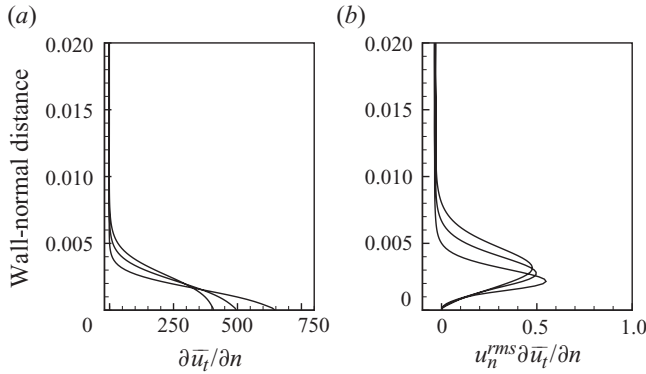
FIGURE 31. Simulation T2, suction surface. (a) Profiles of \partial \bar{u}_t / \partial n and (b) the product u_n^{rms} \partial \bar{u}_t / \partial n . The three curves correspond to three downstream locations, x/L = \{0.05, 0.10, 0.15\} .
