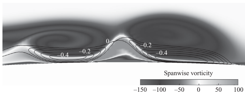
FIGURE 44. Simulation T0: contours of the spanwise vorticity on the suction surface. The snapshot corresponds to the marked region in figure 6(d). The lines mark contours of the tangential velocity.
