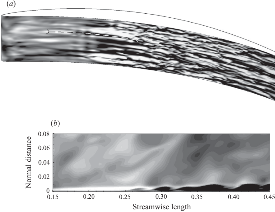
FIGURE 22. Simulation T1. (a) Plane and (b) side views of the tangential perturbation field, -0.1 < u'_t < 0.1 , at the intermediate time in figure 21. The plane view shows that the instability occurs near the upstream edge of the low-speed streak and the downstream edge of the high-speed streak. The dashed line marks the location of the side view (b). The side-view plane bisects the disturbance wave which leads to breakdown.
