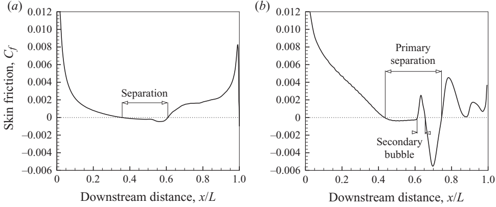
FIGURE 4. Simulation T0: skin friction on (a) the pressure and (b) suction surfaces of the blade. The separation regions are marked.
