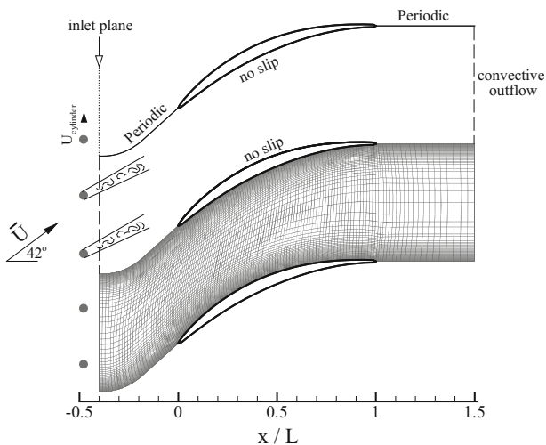
Fig. 1 Upper part: Cross section through the computational domain at midspan. Lower part: Computational grid, showing every 8 th line in x and y
