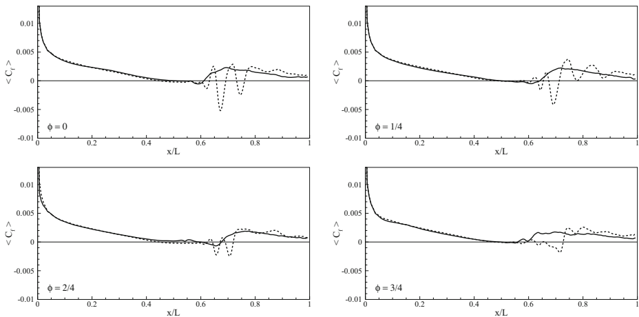
Fig. 14 Phase-averaged friction coefficient ( C_f ) along the suction surface at phases \phi = 0, 1/4, 2/4, 3/4 . Simulations W1 (---) and W2 (—)
