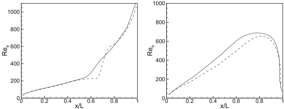
Fig. 8 Time-averaged Re_\theta along the suction surface (left pane) and the pressure surface (right pane). Simulations W1 (---) and W2 (—)
