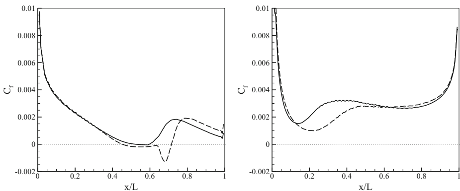
Fig. 6 Time-averaged skin friction coefficient around the suction surface (left pane) and the pressure surface (right pane). Comparison of simulation W2 (—) with simulation W1 (---) - with lower intensity wakes
