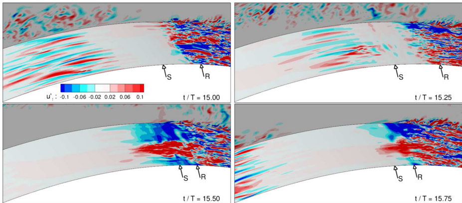
Fig. 17 Simulation W2: Evolution of the tangential velocity fluctuations in a wall-parallel surface inside the suction side boundary layer at four different times. The plane at the back shows the spanwise velocity fluctuations to identify the location of the wakes. The arrows identify the locations of boundary layer separation (S) and reattachment (R)
