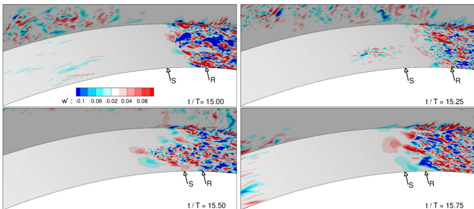
Fig. 18 Simulation W2: Evolution of the spanwise velocity fluctuations in a plane in the suction side boundary layer at four different times. The plane at the back also shows the spanwise velocity fluctuations to identify the location of the wake, the arrows identify the phase-averaged locations of boundary layer separation (S) and reattachment (R)
