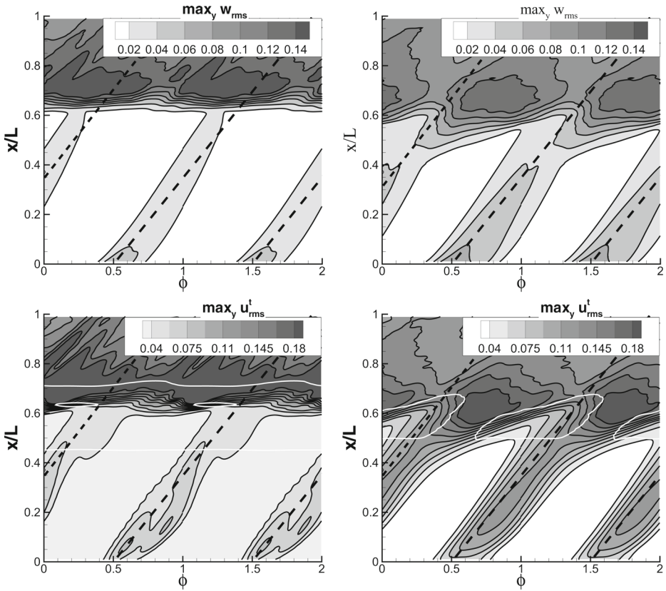
Fig. 15 \max_y(u'_{rms}) and (w_{rms}) along suction surface versus phase ( carpet plot ). Left: weak wakes (W1), right: strong wakes (W2). The white contour in the \max_y(u'_{rms}) plots from simulations W1 & W2 identifies separation. As in Fig. 10, the dashed lines correspond to the location of the wakes at the edge of the boundary layer.
