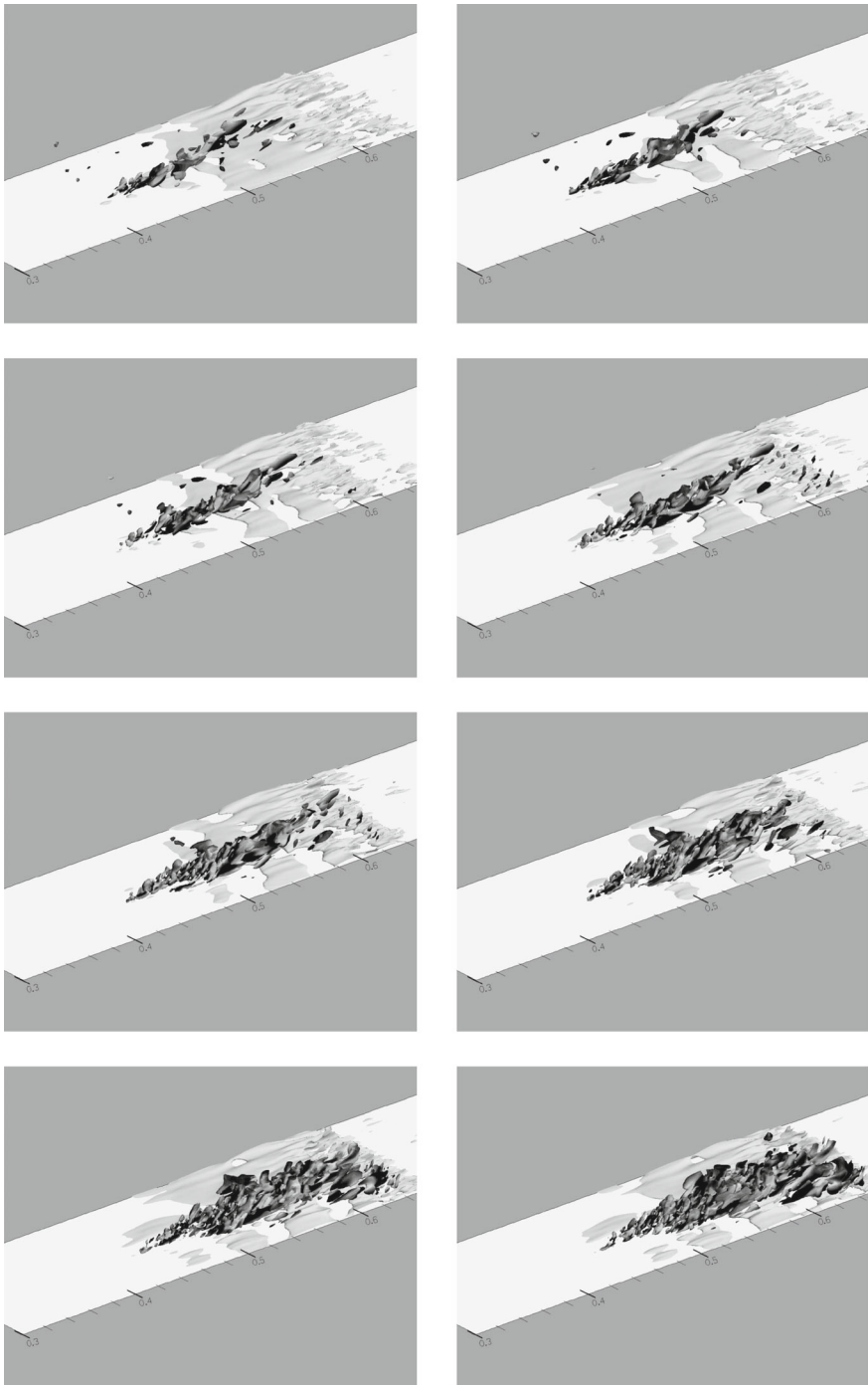
Fig. 20 Simulation W2: A sequence of snapshots illustrating the movement of a turbulent spot ( dark isosurfaces ) through a separation bubble ( light isosurface ). The dark isosurfaces correspond to a wall-normal velocity of \pm 0.1 U and the light-gray isosurface corresponds to zero tangential velocity
