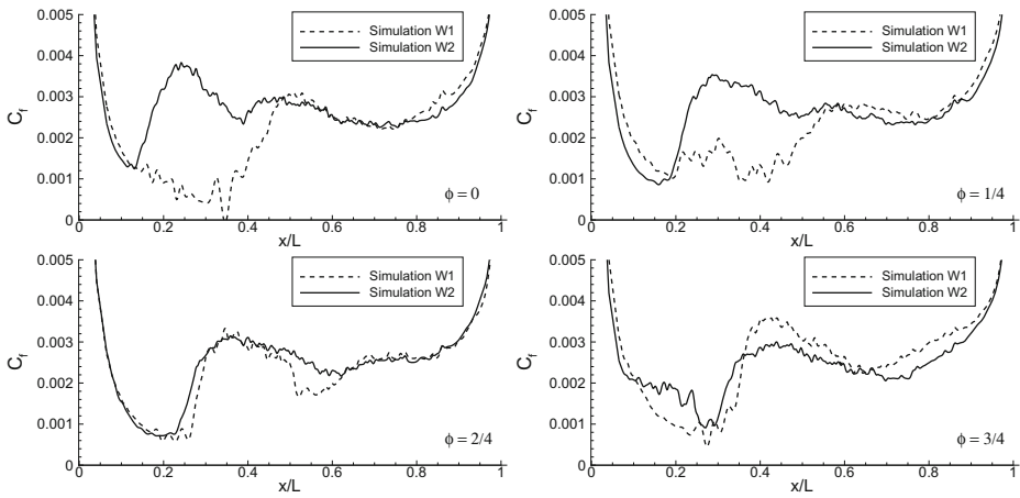
Fig. 9 Phase-averaged friction coefficient along the pressure side from Simulations W1 and W2. The actual location of the wakes can be seen in Fig. 2
