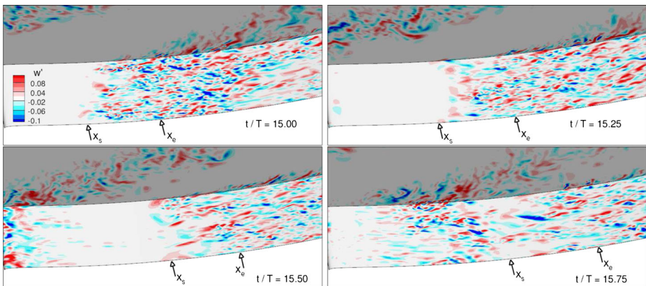
Fig. 13 Simulation W2: Evolution of the spanwise velocity fluctuations in a plane in the pressure side boundary layer at four different times. The plane at the back shows the spanwise velocity fluctuations to identify the location of the wakes. The arrows indicate the location of the start and end of transition as observed in the phase-averaged statistics
