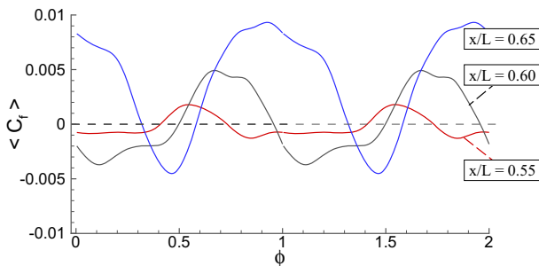
Fig. 16 \langle C_f \rangle versus phase at three locations along the suction surface from simulation W2
