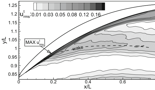
Fig. 11 Simulation W2: Contours of \langle u_{rms}^t \rangle along the pressure surface at \phi = 7/8
