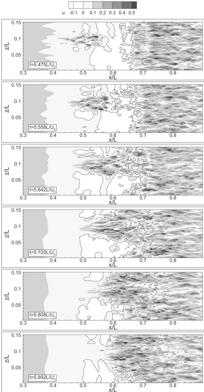
Fig. 19 Simulation W2: A sequence of snapshots showing the evolution a turbulent spot as it is convected through a separation bubble in simulation W2. The figures shows contours of the tangential velocity in a surface at a distance 0.00089L from the suction surface. The black curve identifies the region where the flow is separated
