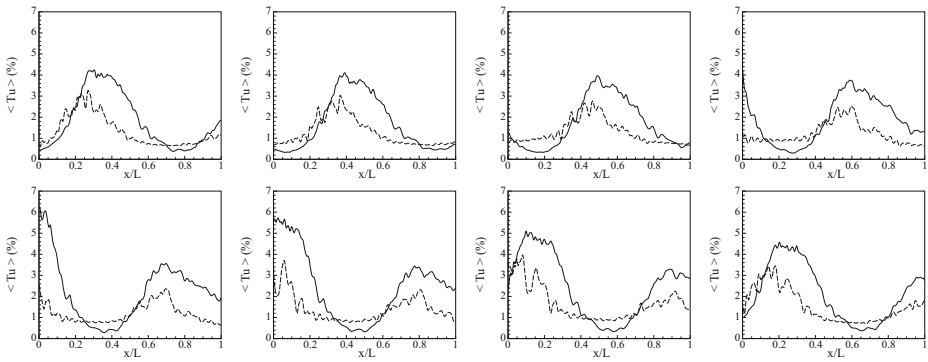
Fig. 3 Phase-averaged turbulent intensity at mid-pitch at eight phases, \phi = 0, 1/8, 2/8, \dots, 7/8 . Comparison of simulation W2 (—) with simulation W1 (---) with lower intensity wakes
