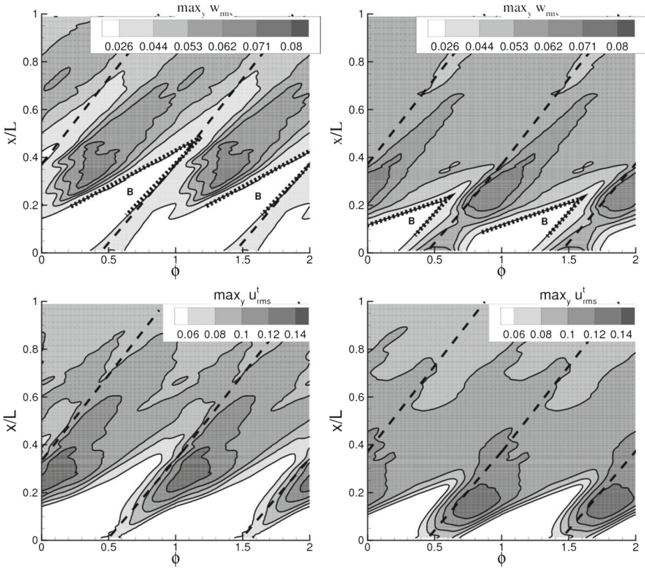
Fig. 10 Contours of \max_y \langle w_{rms} \rangle (upper part) and \max_y \langle u_{rms}^t \rangle (lower part) along the pressure surface (carpet plots). Left: weak wakes, right: strong wakes. The location of the wakes at the edge of the boundary layer is identified by the dashed lines, The border of the becalmed region, labelled “B”, is identified in the \max_y \langle w_{rms} \rangle plots by the thick dotted lines
