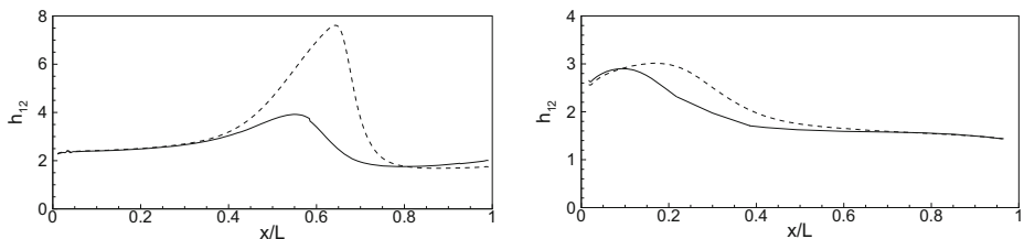
Fig. 7 Time-averaged shape factor along the suction surface ( left pane ) and the pressure surface ( right pane ). Simulations W1 (---) and W2 (—)
