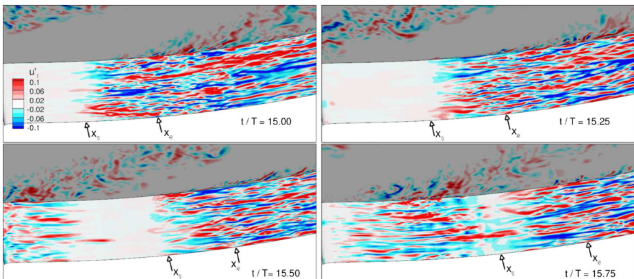
Fig. 12 Simulation W2: Evolution of the tangential velocity fluctuations in a plane in the pressure side boundary layer at four different times. The plane at the back shows the spanwise velocity fluctuations to identify the location of the wakes. The arrows indicate the location of the start and end of transition as observed in the phase-averaged statistics, see also Fig. 9
