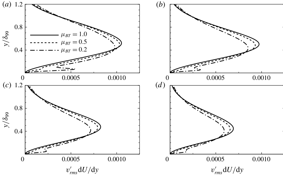
FIGURE 10. Profiles of v'_{rms} dU/dy for (a) x - x_0 = 50 , (b) x - x_0 = 100 , (c) x - x_0 = 150 and (d) x - x_0 = 200 .
