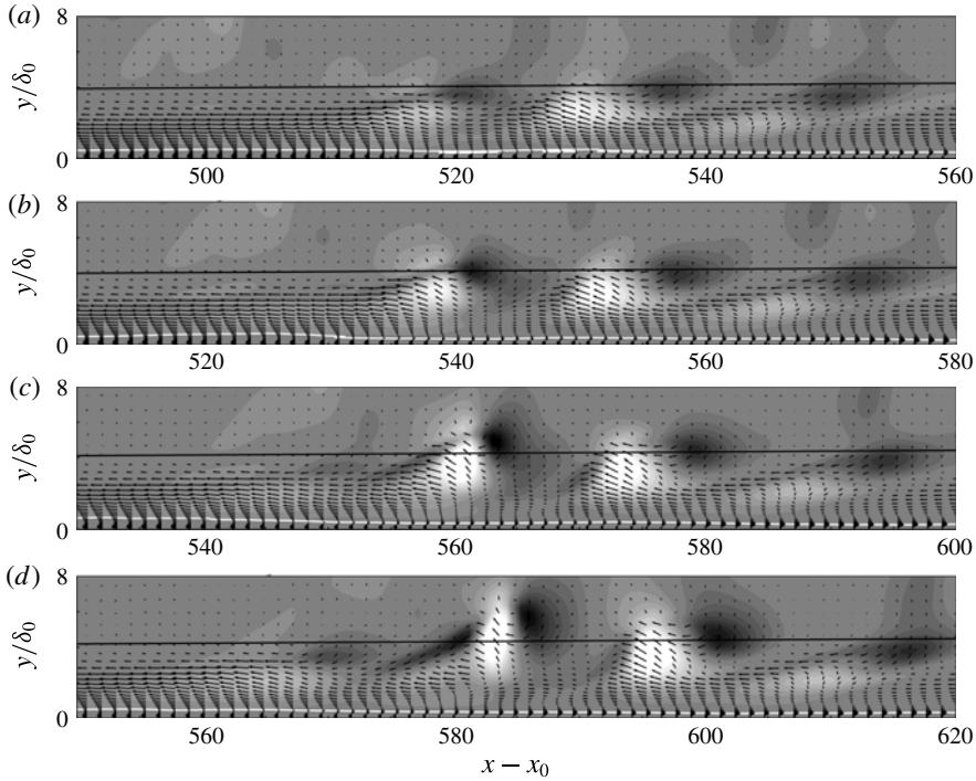
FIGURE 14. Instantaneous v' contours ( -0.05U_\infty < v' < 0.05U_\infty ) in the (x, y) -plane for \mu_{BT} = 0.2 . Time sequence showing the evolution of the spot precursor via vectors: (a) T_0 ; (b) T_0 + \Delta T ; (c) T_0 + 2\Delta T ; (d) T_0 + 3\Delta T . Black and white lines denote the locations of the boundary-layer edge and the interface, respectively. The viewing window moves at 0.83U_\infty . Here, \Delta T = 24\delta_0/U_\infty .
