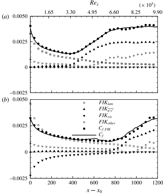
FIGURE 4. Contributions to the Skin friction coefficients for (a) \mu_{BT} = 1.0 and (b) \mu_{BT} = 0.2 .
