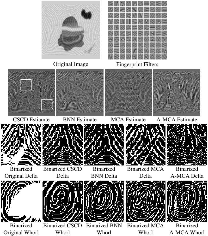
Figure 6: Fingerprint separation results. We compare the visual performance of our method with that of BNN, MCA and A-MCA based om recovered Whor and Delta part.
