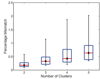
Fig. 2. Nyström clustering consistency for N_s = 2,000 . The red lines indicate median values, the box corresponds to the upper and lower quartiles, and error bars denote the 10^{th} and 90^{th} percentiles.
