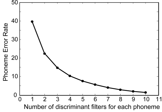
Figure 3. Phoneme error rate on the training examples vs. the number of spectrotemporal filter sets used. Each set is optimized for the classification of the samples that were not correctly recognized by the previous sets.
