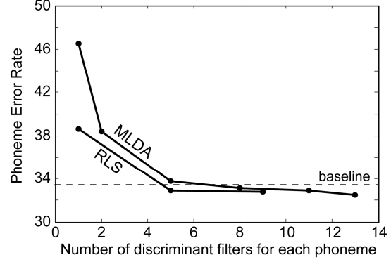
Figure 4. Phoneme error rate vs. number of feature sets obtained from MLDA and RLS algorithms. The system from RLS reaches a better performance for the same number of features; they both converge to about the same performance.
